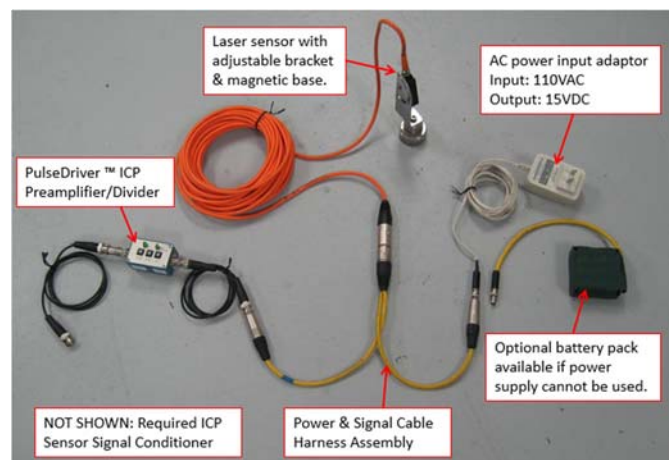
Figure 2. Light Tach Kit General Configuration
